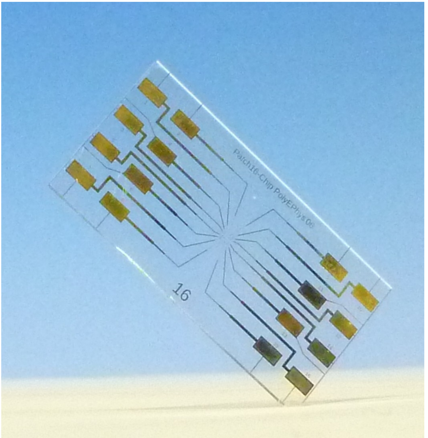
The result of long-term cooperation: the chip is a biohybrid sensor consisting of biological and microtechnical parts. The biological pores are only a few nanometres in diameter and cannot be seen with the naked eye. © Dr. Gerhard Baaken
