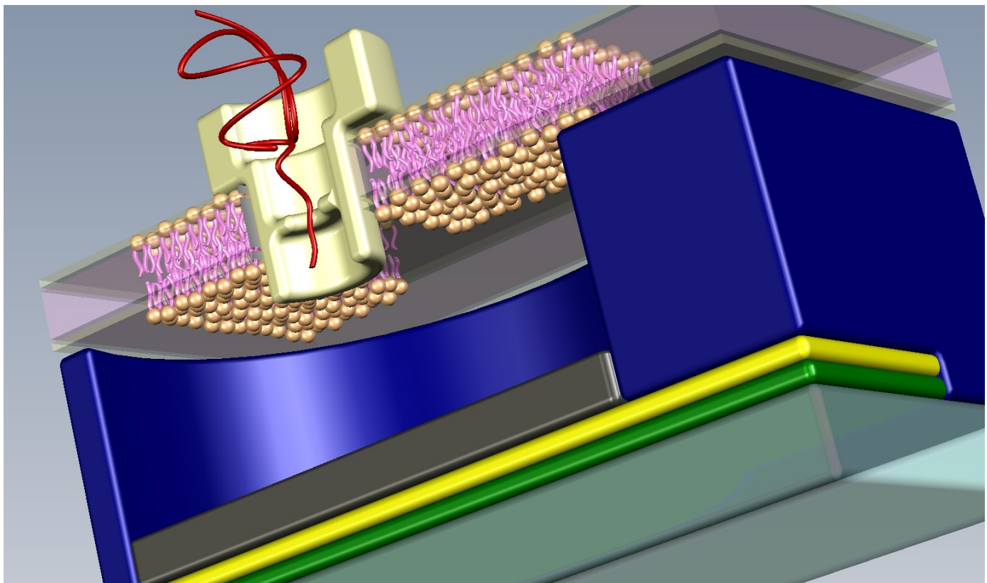
Principle of a chip with a biological nanopore for determining the chain length of polymer molecules.
